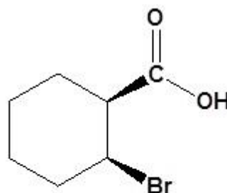
Cis -2-Bromocyclohexanecarboxylic acid
