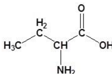
2-Aminobutanoic acid
