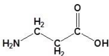
3-Aminopropanoic acid
