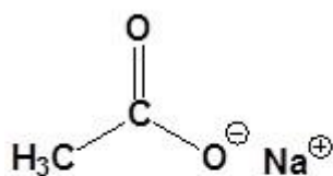
Sodium ethanoate
