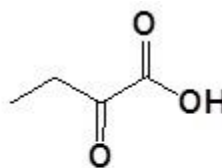
2-Oxobutanoic acid
