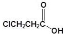
3-Chloropropanoic acid (γ-Chloropropionic acid)
