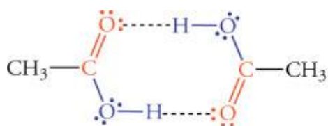
Hydrogen-bonded dimer of acetic acid
