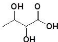
2,3-Dihydroxybutanoic acid
