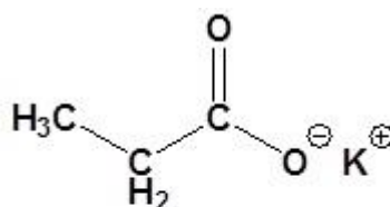
Potassium Propanoate
