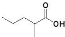
2-Methylpentanoic acid (β-Methylvaleric acid)
