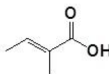
( E )-2-Methyl-2-butenoic acid
